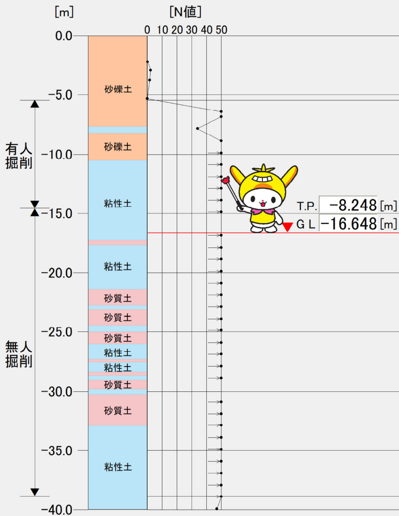
[土質柱状図]
