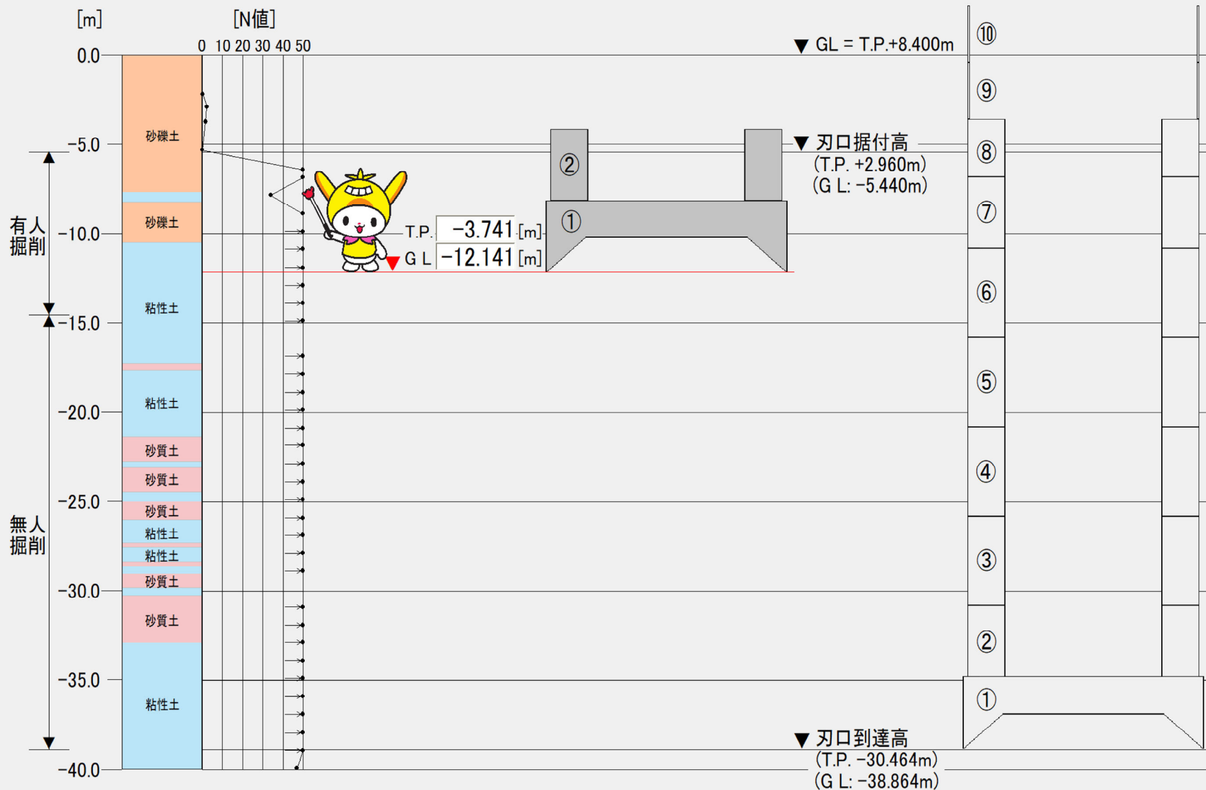
[土質柱状図]
